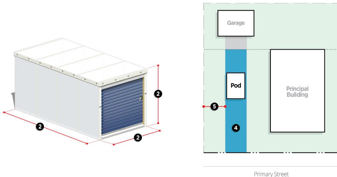
Figure 4.12: Portable Storage Structure (POD) Standards
