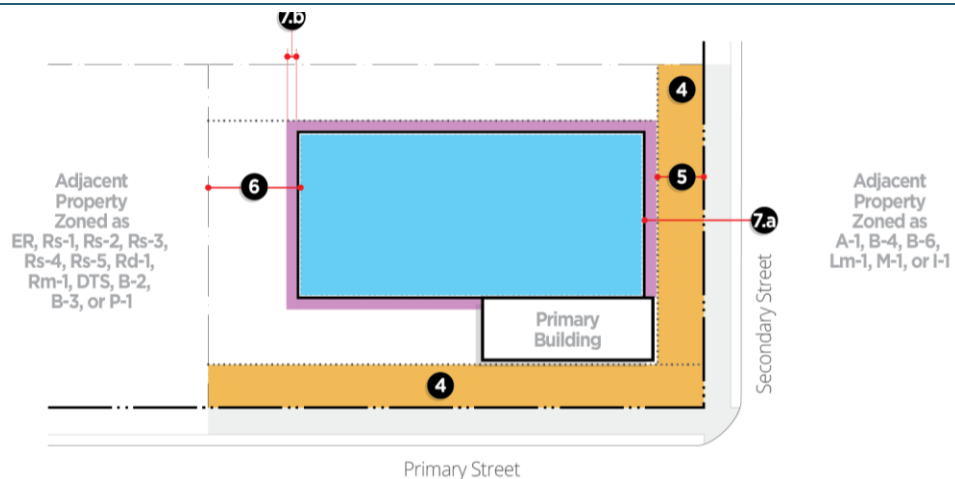
Figure 4.7: Outdoor Activity/Operations Standards
