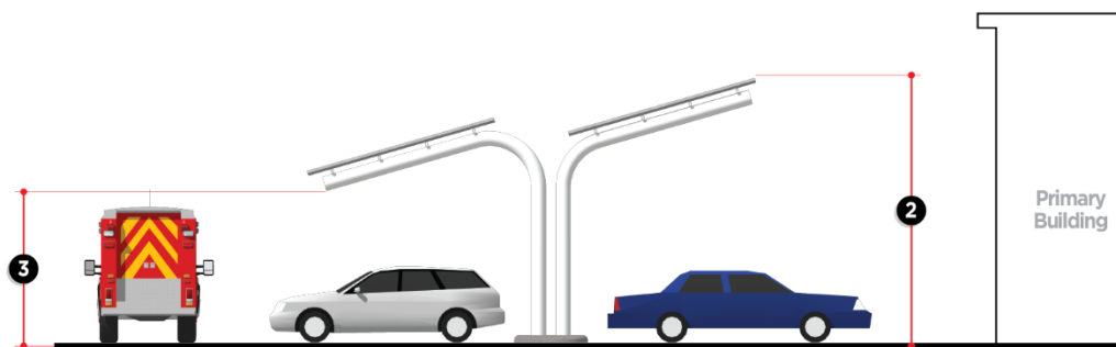
Figure 4.8: Solar Energy Collection System, Canopy Standards
