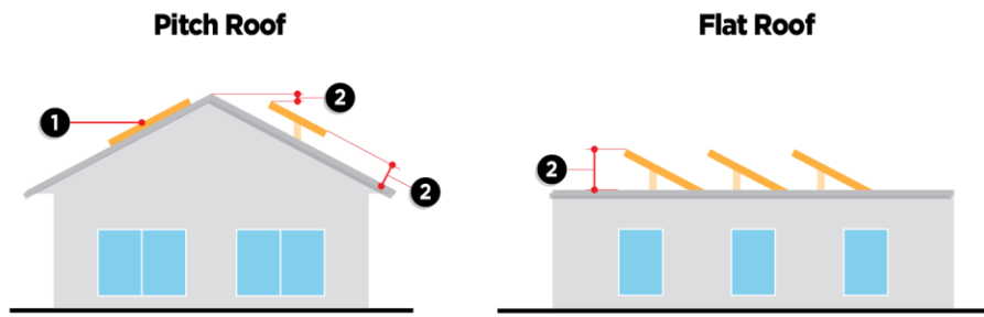
Figure 4.10: Solar Energy Collection System, Roof Mounted Standards
